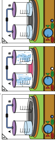
Evaporation and Condensation Cycle
